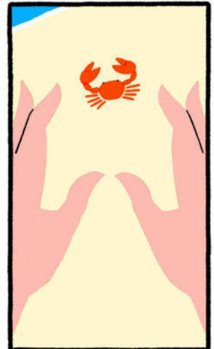
CANCER / CNC
