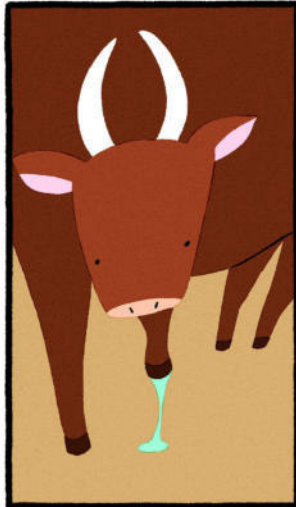
TAURUS / TAU
