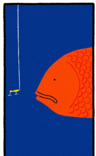
PISCES / PSC
